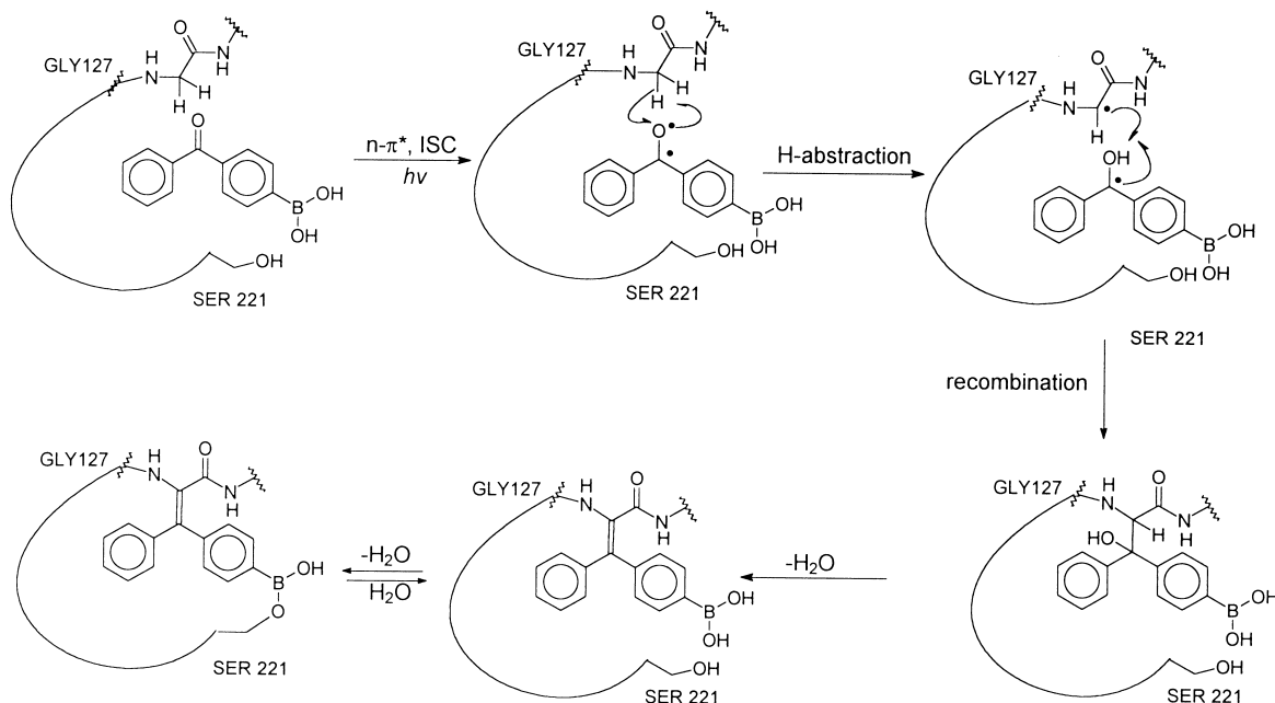
Figure 3. Proposed mechanism of BBP crosslinking: the photoactivated crosslinking of BBP to Gly127 and dehydration. The last dehydration step forming a boronate ester between BBP and the enzyme may precede crosslinking.
