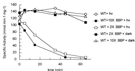
Figure 1. Time course for photolysis (350 nm) of SBL-WT and BBP.
