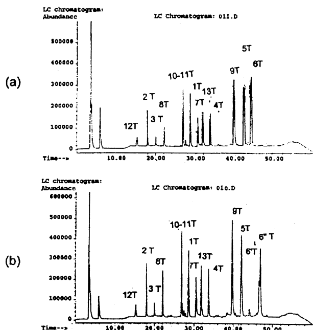
Figure 2. HPLC-trace of (a) native and (b) BBP crosslinked WT-SBL: tryptic fragments 1T–13T are identified.
